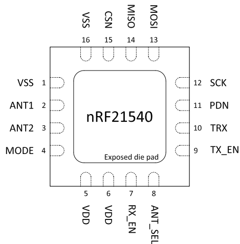
Figure 19: QFN16 pin assignments, top view
