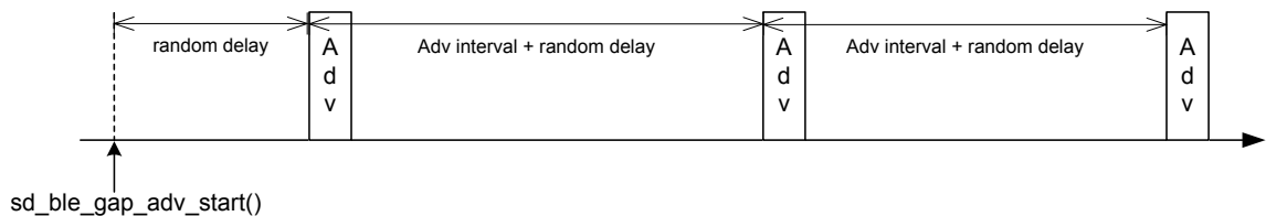
Figure 44: Advertiser
