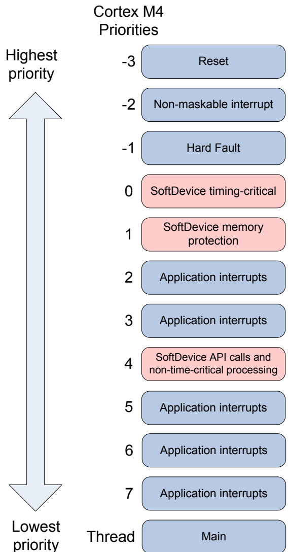
Figure 51: Exception model
