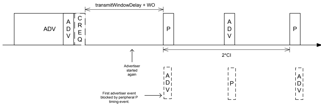
Figure 47: Peripheral connection setup and connection with collision
